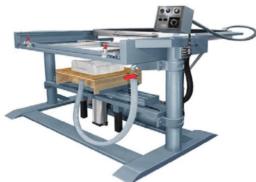
Belovac BV C Class Vacuum Forming Machine
